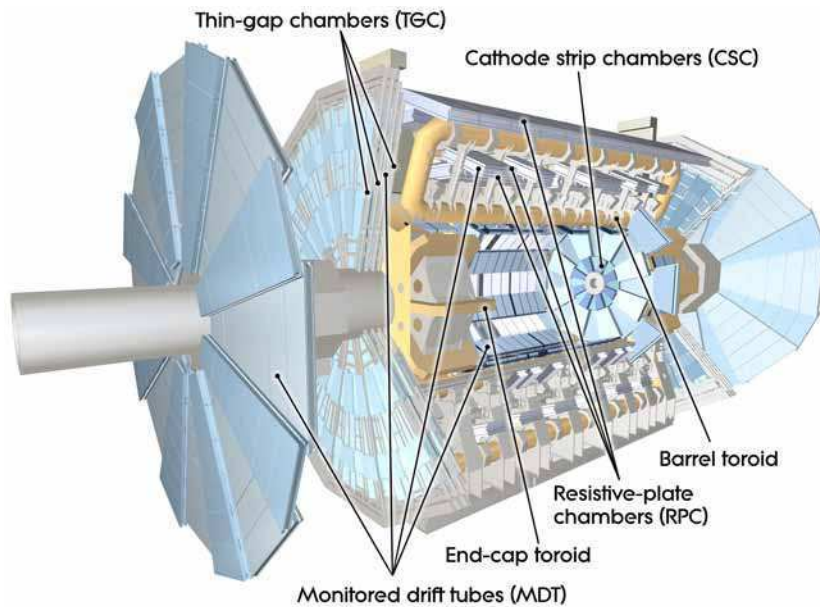
Figure 3.8: The Muon Chamber.
