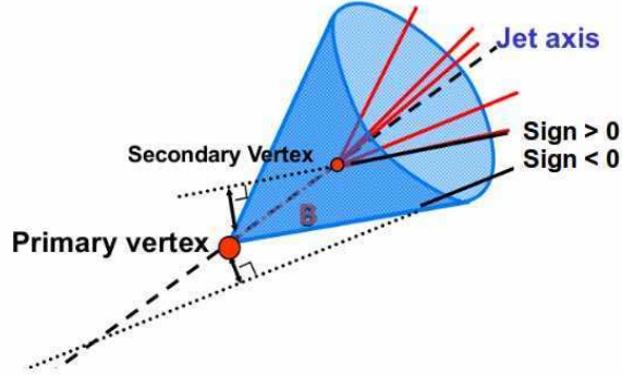
Figure 4.3: Lifetime sign of tracks. A positive and a negative lifetime signed track is shown.
