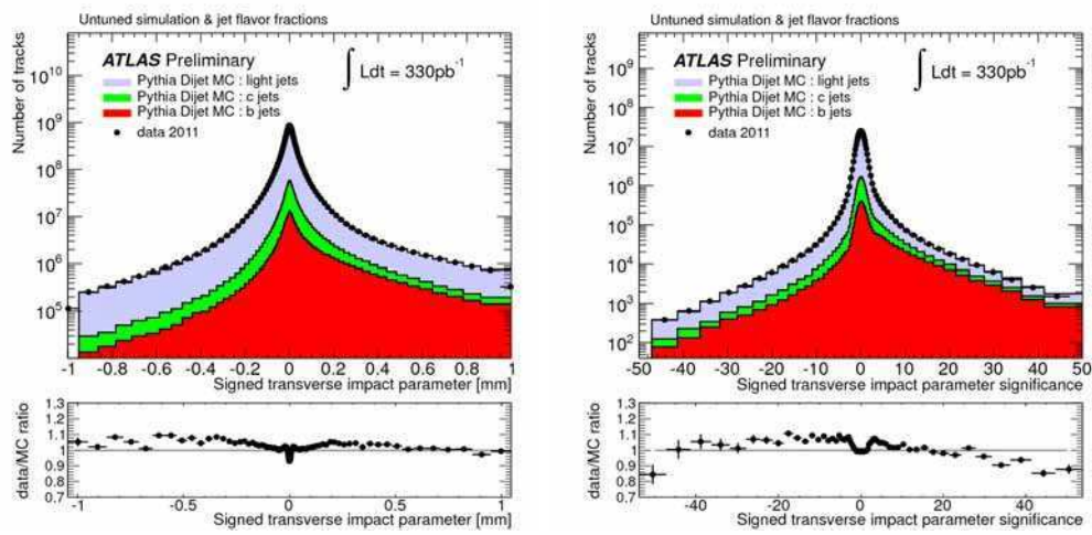
Figure 4.4: Distribution of the signed transverse impact parameter (left) and signed transverse impact parameter significance with respect to primary vertex for tracks associated to jets, for experimental data (solid black points) and for simulated data (filled histograms for the various flavors). The ratio data over simulation is shown at the bottom of the plot.
