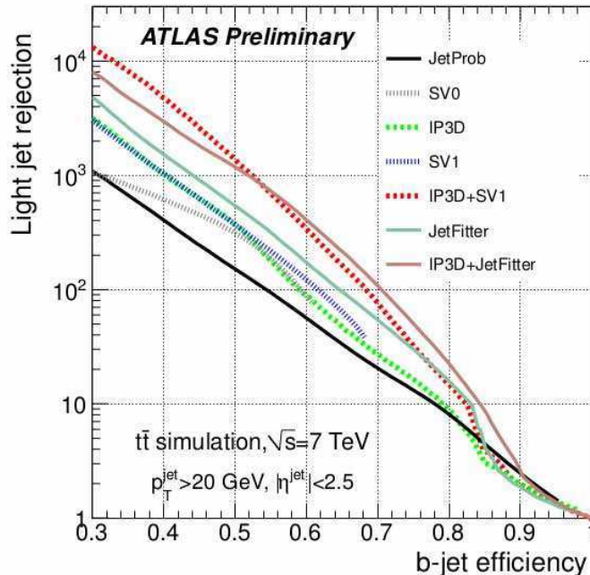
Figure 4.5: Light-jet rejection as a function of the b -jet tagging efficiency for the early tagging algorithms (JetProb and SV0) and for the high-performance algorithms, based on simulated t\bar{t} events.
