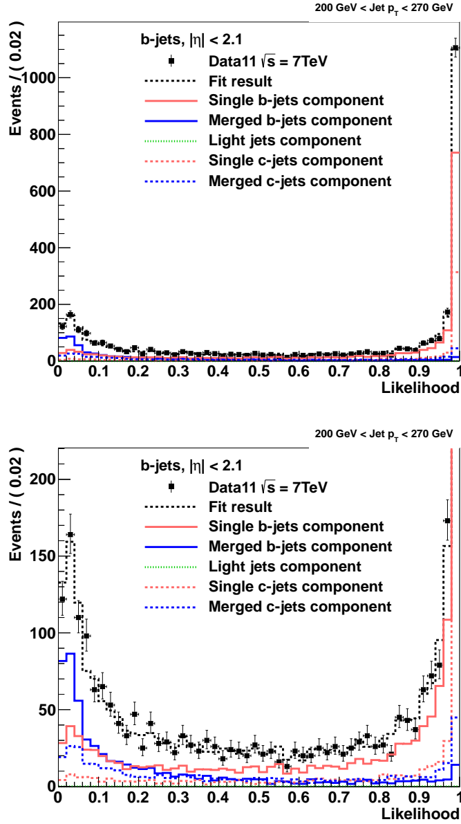
Figure 7.4: Example result of a template fit to the likelihood distribution in data. The result is shown for jets with p_T between 200 GeV and 270 GeV, in full scale (top) and zooming the vertical scale, to better display the flavour content of the data (bottom). Uncertainties shown are statistical only.
