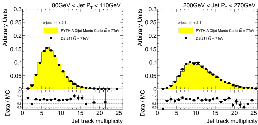
Figure 5.25: Distribution of the jet track multiplicity in 2 different jet p_T bins, for experimental data collected by ATLAS during 2011 (solid black points), and simulated data (filled histograms). Jets were selected using JetFitter tagger at its 60% b -jet efficiency working point. The ratio data over simulation is shown at the bottom of each plot. The agreement is very good.
