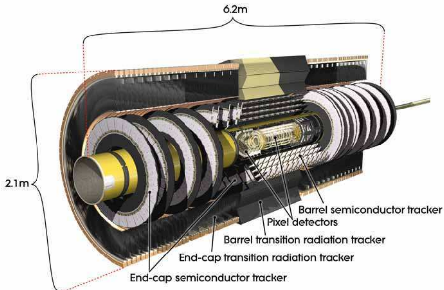
Figure 3.5: Layout of the ATLAS Inner Detector.
