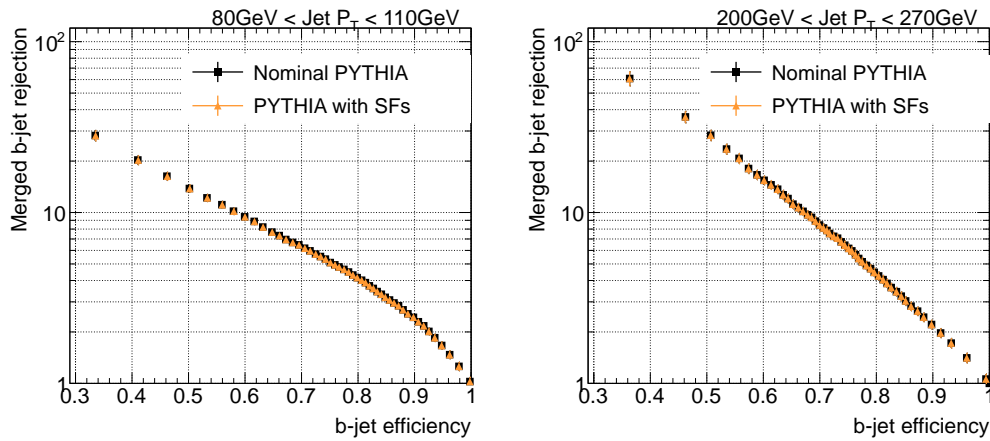
Figure 6.8: Rejection of merged b -jets as a function of single b -jet efficiency with and without scale factors as weights.
