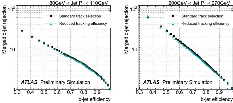
Figure 6.9: Rejection of merged b -jets as a function of the single b -jet efficiency showing shift in likelihood performance caused by a reduction in the tracking efficiency.
