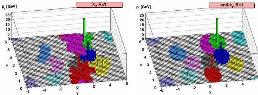
Figure 2.2: A sample parton-level event, generated with HERWIG, clustered with the k_t and anti- k_t algorithms, illustrating the active area of the resulting jets [42].
