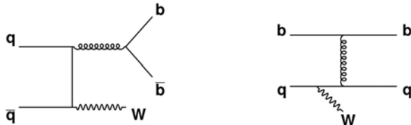
Figure 2.5: Feynman diagrams for W production in association with b quarks.
