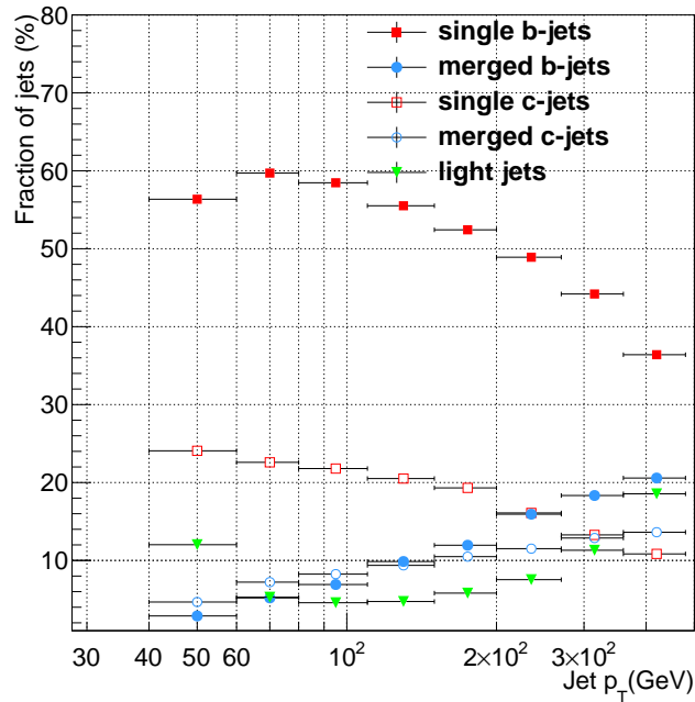
Figure 7.2: Theoretical predictions of the fractions of b -, b\bar{b} -, c -, c\bar{c} -, and \ell -jets in b -tagged jets from a PYTHIA simulation of QCD jet production.
