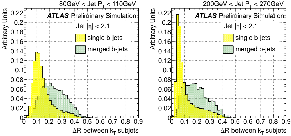
Figure 5.13: Distribution of the \Delta R between the axes of the two k_t subjects in the jet for single and merged b -jets from 80 GeV to 110 GeV (left) and 200 GeV to 270 GeV (right).
