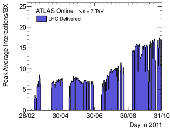
Figure 3.2: The maximum mean number of events per beam crossing versus day in 2011.
