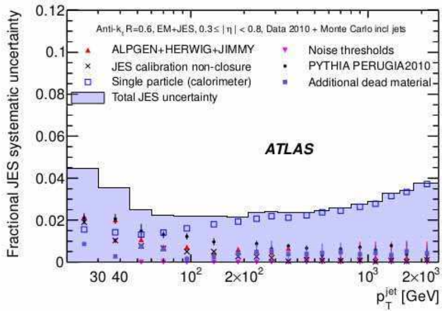
Figure 4.1: Fractional jet energy scale uncertainty as a function of jet p_T for jets in the pseudorapidity region 0.3 < |\eta| < 0.8 in the calorimeter barrel. The total uncertainty is shown as the solid tight blue area. The individual sources are also shown.
