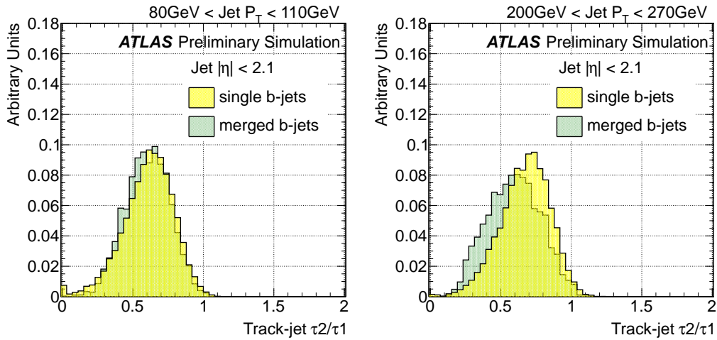
Figure 5.17: Distribution of \tau_2/\tau_1 for single and merged b -jets from 80 GeV to 110 GeV (left) and 200 GeV to 270 GeV (right).
