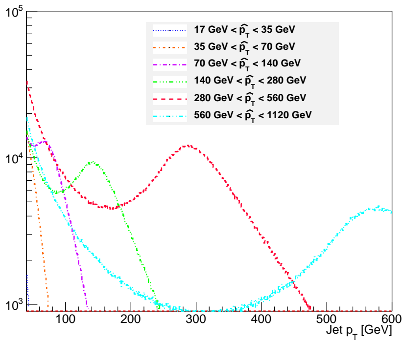
Figure 5.1: Calibrated jet p_T distribution for anti- k_t jets in a dijet Monte Carlo sample composed of different sub-samples generated with increasing thresholds of the hard-scattering partonic transverse momentum, \hat{p}_T .
