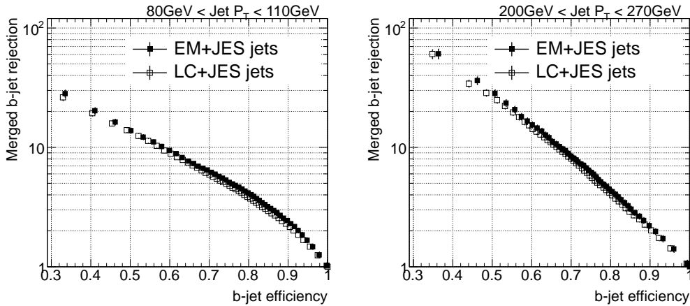
Figure 6.11: Rejection of merged b -jets as a function of single b -jet efficiency for jets calibrated to the EM+JES (LC+JES) scale, between 80 GeV and 110 GeV and 200 GeV and 270 GeV.
