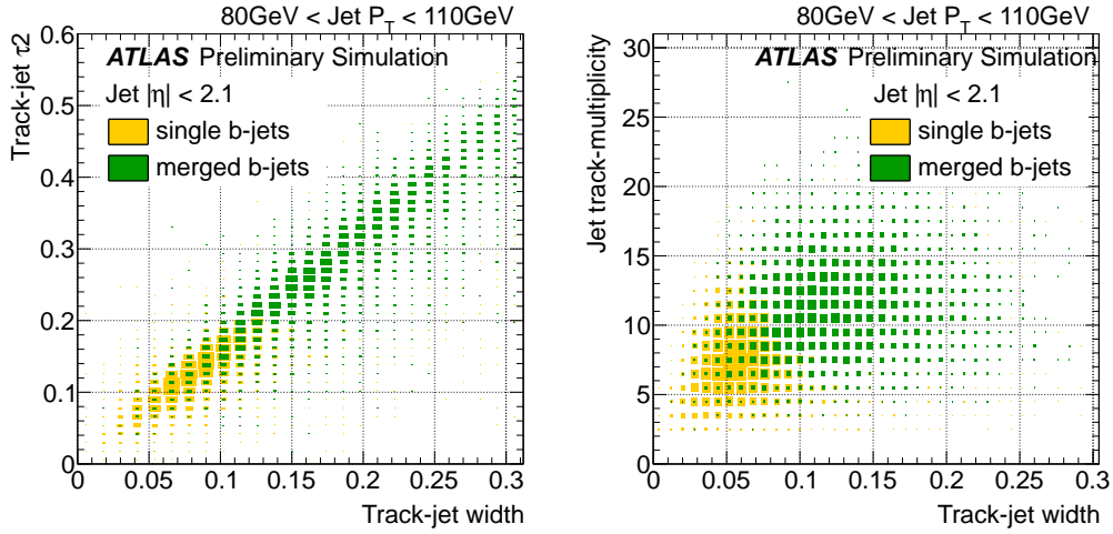
Figure 5.16: Correlation between \tau_2 and track-jet width (left) and jet track multiplicity and track-jet width (right) for single and merged b -jets from 80 GeV to 110 GeV.
