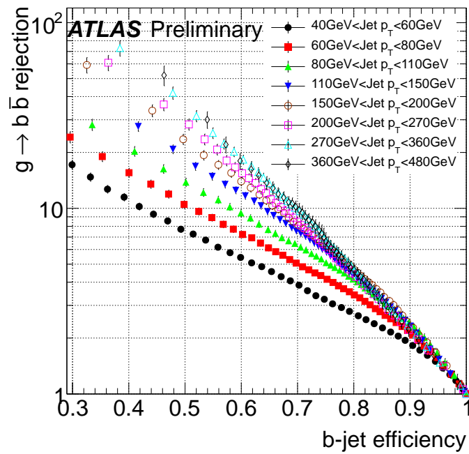
Figure 6.5: Rejection of merged b -jets as a function of single b -jet efficiency for dijet events in 8 jet p_T bins.
