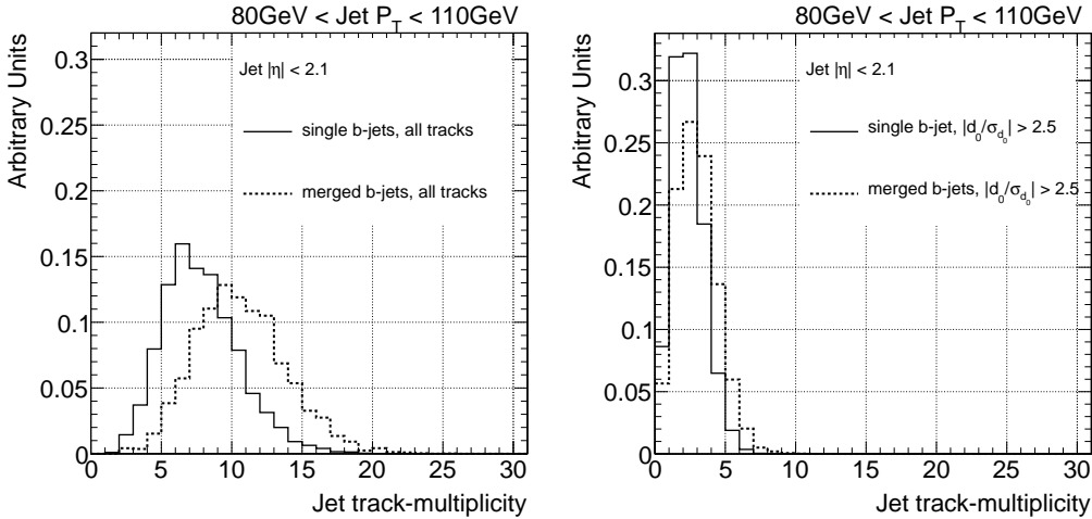
Figure 5.5: Distribution of the jet track multiplicity for single and merged b -jets from 80 GeV to 110 GeV, for all (left) and displaced tracks only (right). No improvement is obtained by using displaced tracks.
