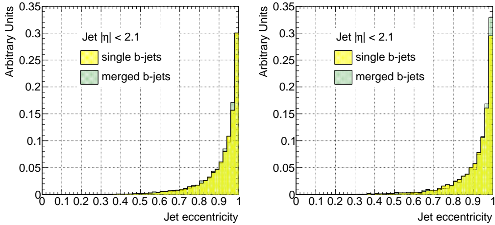
Figure 5.18: Distribution of the jet eccentricity for single and merged b -jets from 80 GeV to 110 GeV (left) and 200 GeV to 270 GeV (right).
