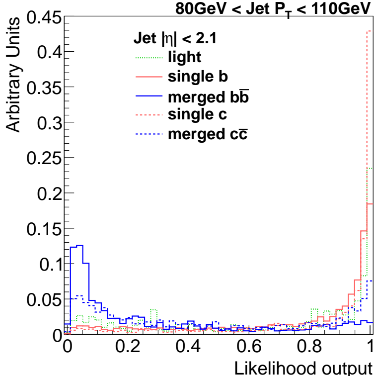
Figure 7.1: Likelihood distribution for the five flavours, b , c , b\bar{b} , c\bar{c} and \ell are shown for b -tagged jets in the simulated QCD sample. The templates are all normalized to unit area to allow the comparison.
