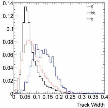
Figure 5.6: Distribution of track-jet width for gluon-initiated ( g ), single ( b ) and merged ( bb ) jets from 80 GeV to 120 GeV in a sample of dijet events generated with PYTHIA and no detector simulation.
