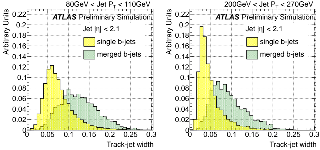
Figure 5.7: Distribution of track-jet width for single and merged b -jets from 80 GeV to 110 GeV (left) and 200 GeV to 270 GeV (right).
