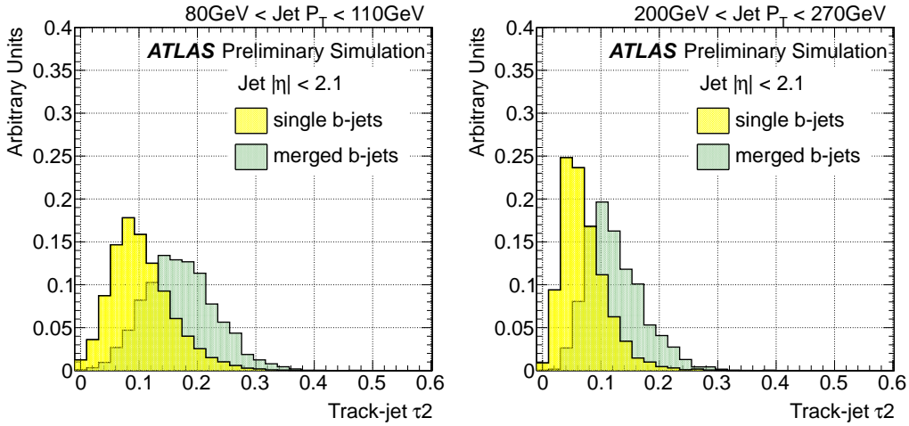
Figure 5.15: Distribution of \tau_2 for single and merged b -jets from 80 GeV to 110 GeV (left) and 200 GeV to 270 GeV (right).
