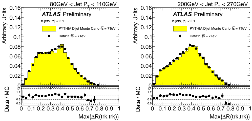
Figure 5.22: Distribution of maximum \Delta R between pairs of tracks in two different jet p_T bins, for experimental data collected by ATLAS during 2011 (solid black points), and simulated data (filled histograms). The ratio data over simulation is shown at the bottom of each plot.
