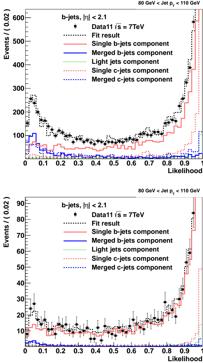
Figure 7.5: Example result of a template fit to the likelihood distribution in the semi-inclusive single- b enriched sample for jets with p_T between 80 GeV and 110 GeV (bottom). The result for the same p_T bin in the inclusive sample is also shown for comparison (top). The vertical scale was enlarged in the two plots to better appreciate all contributions. Uncertainties shown are statistical only.
