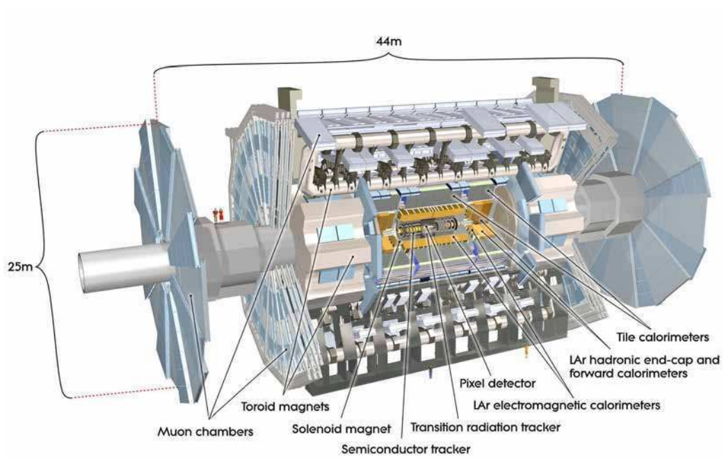
Figure 3.4: The ATLAS Detector.
