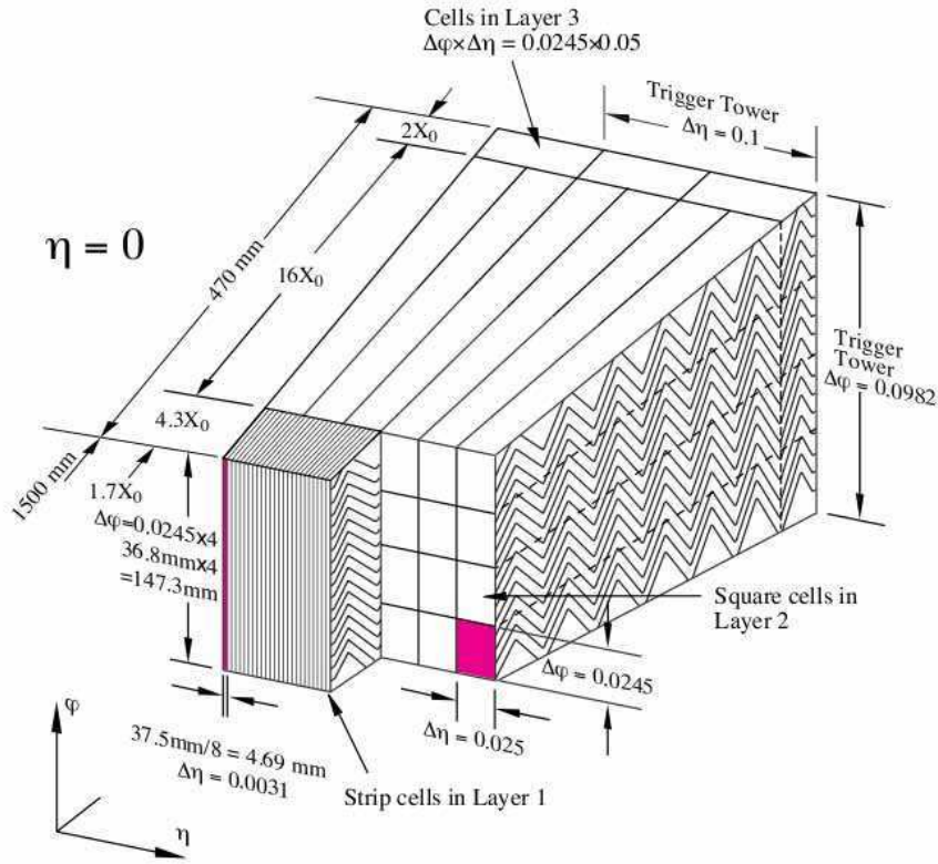
Figure 3.7: Cross section of the LAr barrel calorimeter where the different layers are visible. The granularity in \eta and \phi of the cells of each of the three layers is also shown.
