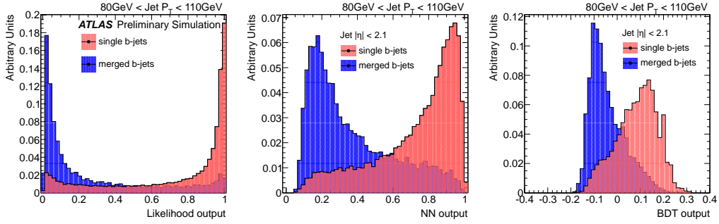
Figure 6.2: Distribution of the MVA discriminant outputs for the Likelihood (a), Neural Network (b) and Boosted Decision Trees (c) classifiers, for single and merged b -jets between 80 GeV and 110 GeV.
