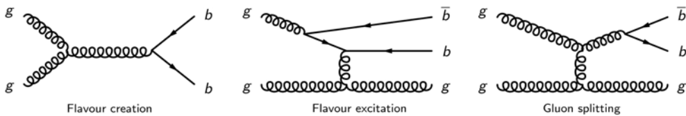
Figure 2.3: Representative diagrams of the three channels contributing to QCD b -quark production up to NLO. (a) Left : The flavour creation channel is the only one present at LO. At NLO, two new channels open up, referred to as (b) Center : flavour excitation (center) and (c) Right : gluon splitting.
