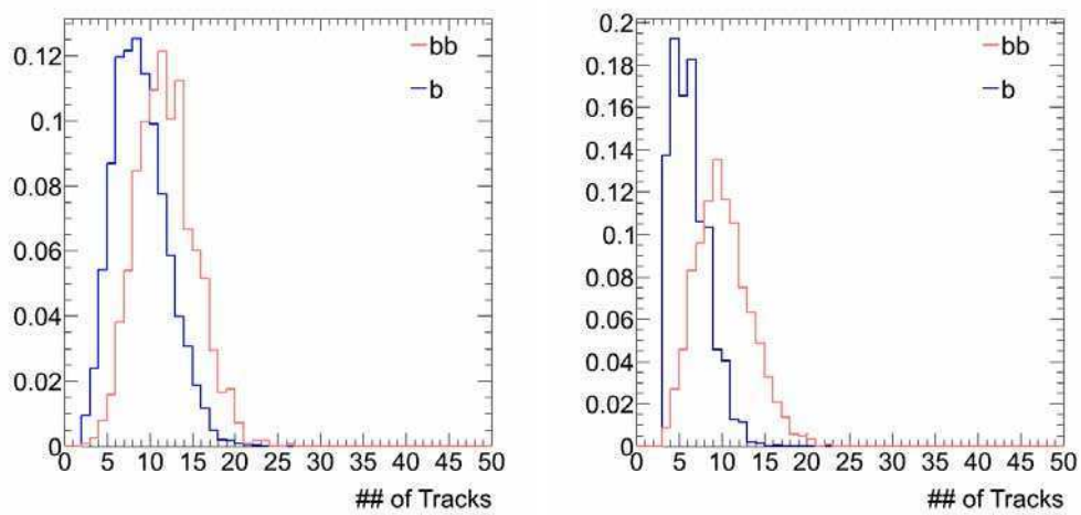
Figure 5.4: Distribution of the charged particle multiplicity for single ( b ) and merged ( bb ) jets from 80 GeV to 120 GeV in a sample of dijet events generated with PYTHIA and no detector simulation. Distributions are shown using all charged particles (left) and using only charged particles coming from b -hadron decay (right). A better discrimination between single and merged b -jets is obtained when using tracks from b -decay only.
