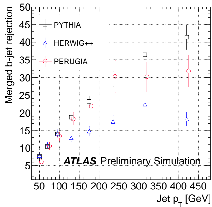
Figure 6.12: Rejection of merged b -jets as a function of jet p_T for different Monte Carlo generators, at the 50% efficiency working point. The Perugia points are shifted by +5 GeV for display purposes.
