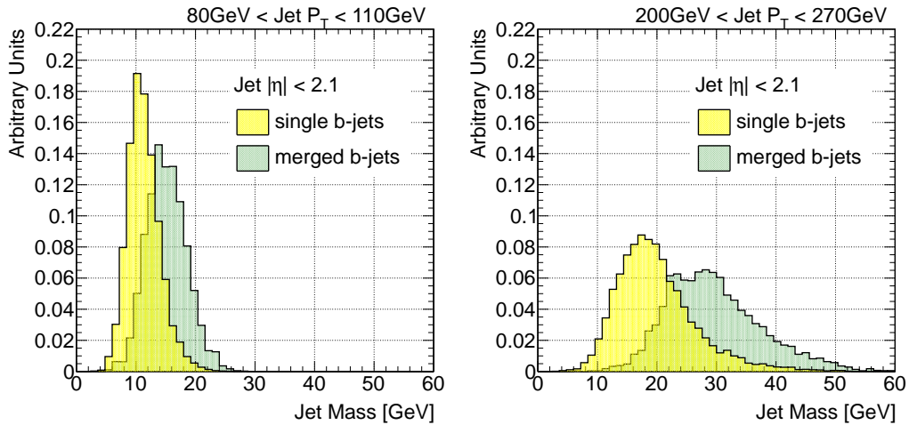
Figure 5.9: Distribution of jet mass in GeV for single and merged b -jets from 80 GeV to 110 GeV (left) and 200 GeV to 270 GeV (right).
