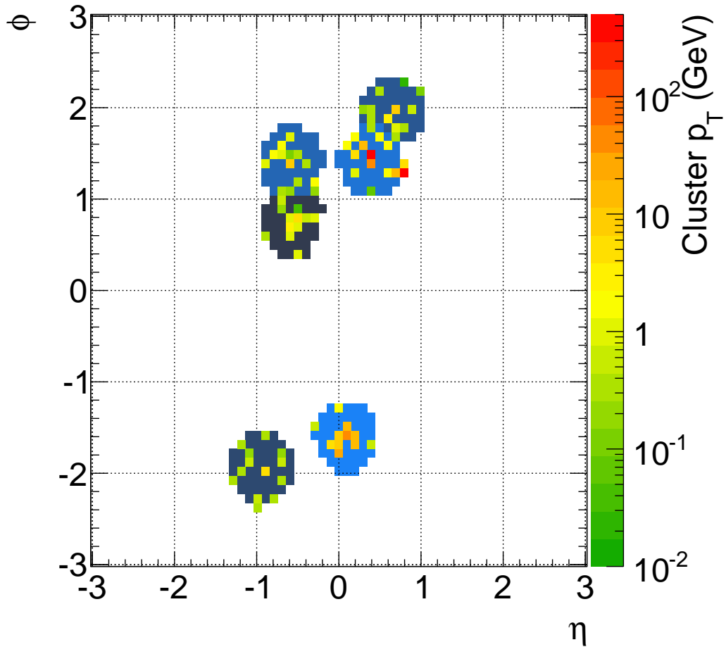
Figure 5.14: Event display of a merged b -jet in (\eta, \phi) = (0.46, 1.41) and p_T = 110 GeV. The two b -hadrons are indicated as two red squares. The area of the jet is shown in blue and the topoclusters belonging to the jet are shown in different colors, from green to orange, depending on their transverse momentum. The \Delta R between the axes of the two k_t subjets in the jet is larger than 0.3. The two-subjet structure of the merged jet is displayed.
