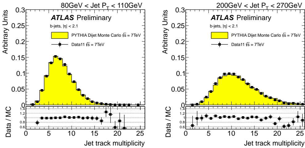
Figure 5.19: Distribution of the jet track multiplicity in 2 different jet p_T bins, for experimental data collected by ATLAS during 2011 (solid black points), and simulated data (filled histograms). The ratio data over simulation is shown at the bottom of each plot.
