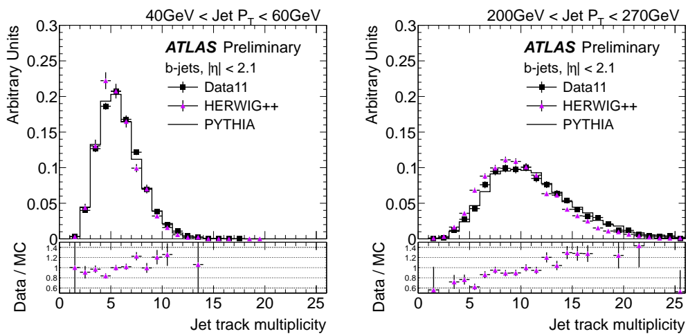
Figure 6.13: Distribution of the jet track multiplicity in 2 different jet p_T bins, for experimental data collected during 2011 (solid black points) and HERWIG++ events (solid violet triangles). The ratio data over HERWIG++ simulation is shown at the bottom of the plot. PYTHIA distribution is also shown for reference.
