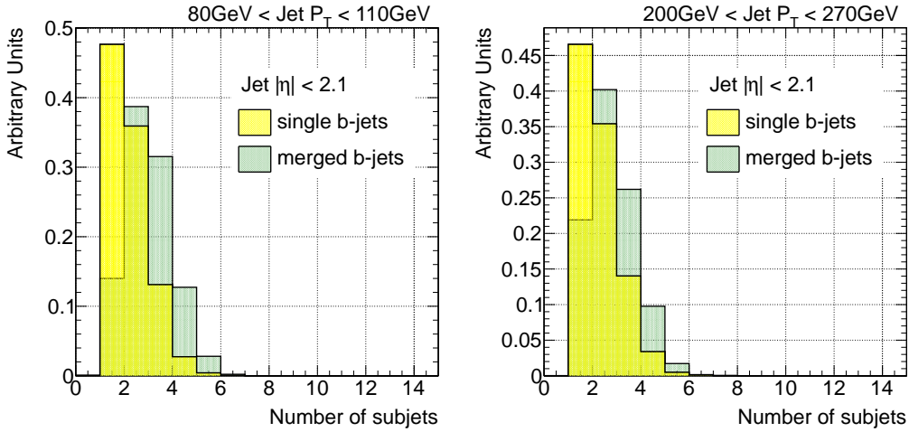
Figure 5.12: Distribution of the number of k_t sub-track-jets for single and merged b -jets from 80 GeV to 110 GeV (left) and 200 GeV to 270 GeV (right).
