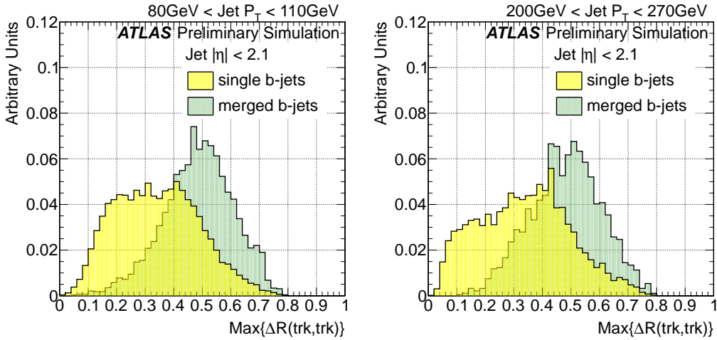
Figure 5.11: Distribution of the maximum \Delta R between pairs of tracks for single and merged b -jets from 80 GeV to 110 GeV (left) and 200 GeV to 270 GeV (right).
