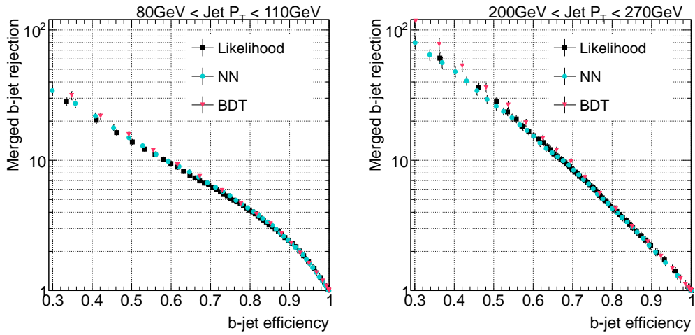
Figure 6.3: Rejection of merged b -jets as a function of single b -jet efficiency for the the different MVA methods evaluated for medium and high jet p_T .
