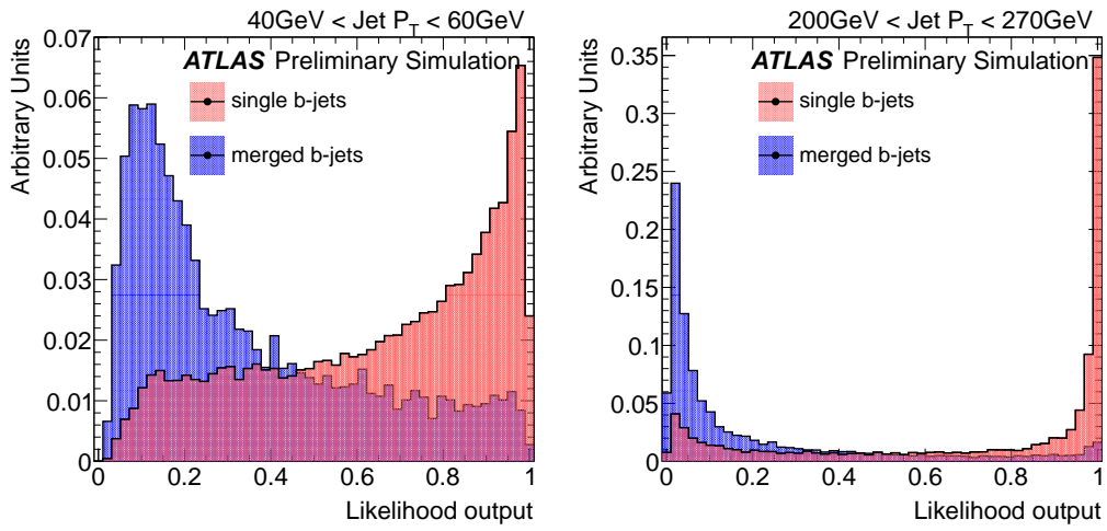
Figure 6.4: Distribution of the likelihood output for single and merged b -jets for low and high p_T jets.
