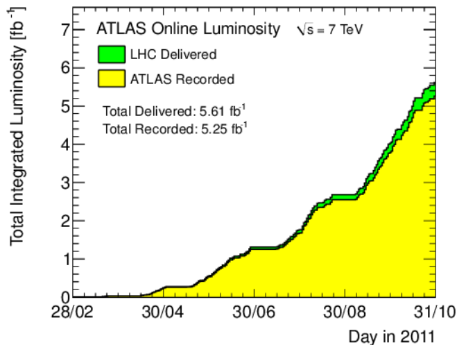
Figure 3.3: Total luminosity delivered by the LHC and recorded by ATLAS during the 2011 \sqrt{s} = 7 TeV proton-proton run.
