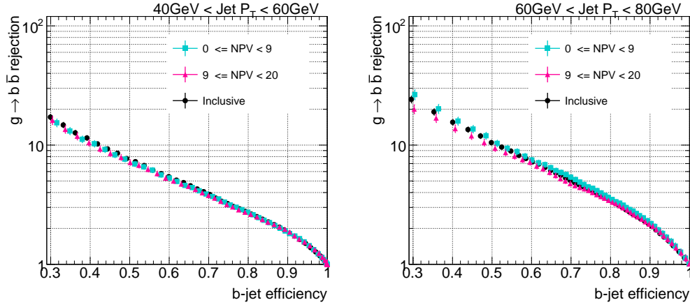
Figure 6.6: Rejection of merged b -jets as a function of single b -jet efficiency in bins of NPV for two low jet p_T bins.
