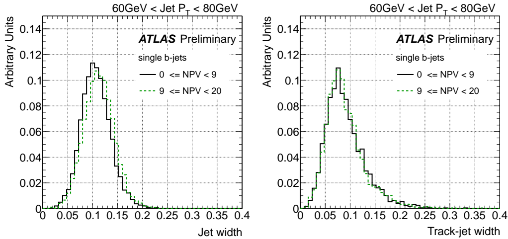
Figure 5.8: Distribution of jet width using topological clusters (left) and tracks (right) for single b -jets in two bins of number of primary vertices (NPV) for jets from 60 GeV to 80 GeV.
