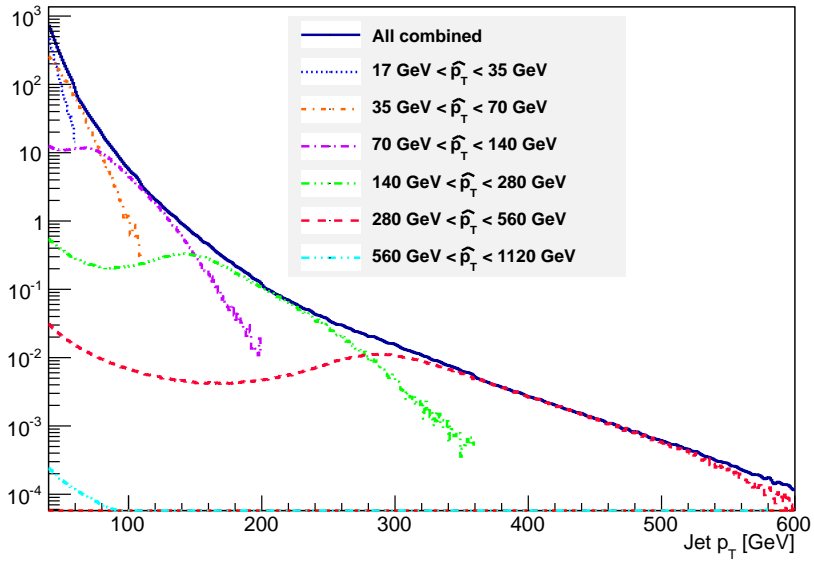
Figure 5.2: Calibrated jet p_T distribution for anti- k_t jets in a dijet Monte Carlo sample composed of different sub-samples generated with increasing thresholds of the hard-scattering partonic transverse momentum, \hat{p}_T . In order to obtain the falling p_T spectrum observed in data, the different samples were weighted by their respective production cross sections.
