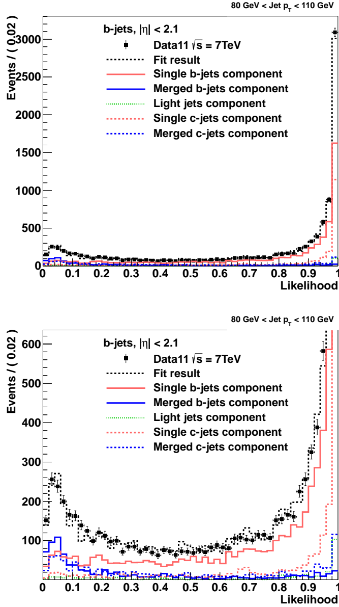
Figure 7.3: Example result of a template fit to the likelihood distribution in data. The fit is shown for jets with p_T between 80 GeV and 110 GeV, in full scale (top) and zooming the vertical scale, to better display the flavour content of the data (bottom). Uncertainties shown are statistical only.
