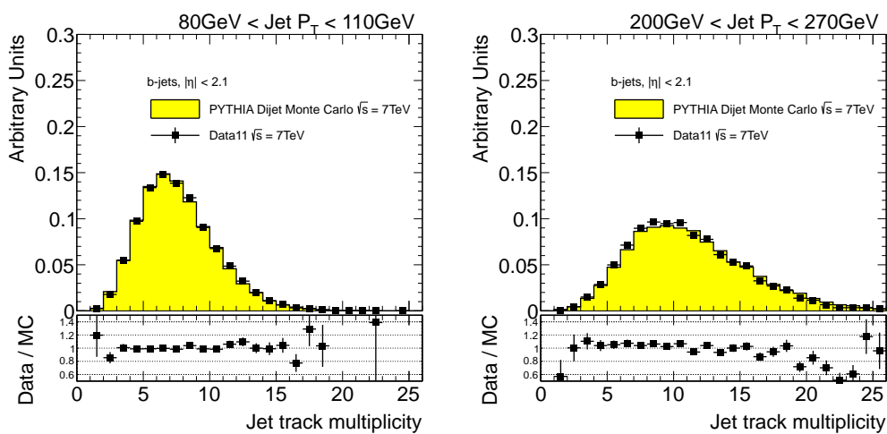
Figure 5.24: Distribution of the jet track multiplicity in 2 different jet p_T bins, for experimental data collected by ATLAS during 2011 (solid black points), and simulated data (filled histograms). Jets were selected using MV1 tagger at its 70% b -jet efficiency working point. The ratio data over simulation is shown at the bottom of each plot. The agreement is very good.
