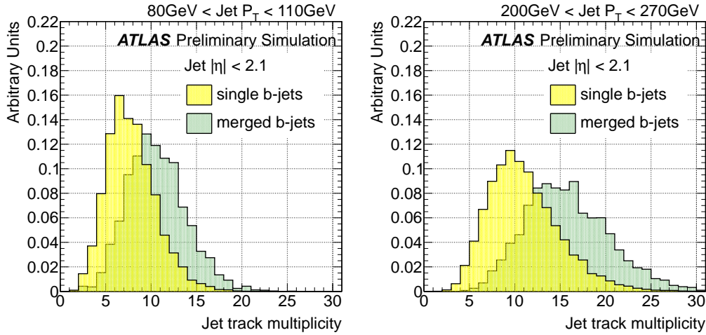
Figure 5.3: Distribution of the track multiplicity for single and merged b -jets from 80 GeV to 110 GeV (left) and 200 GeV to 270 GeV (right).
