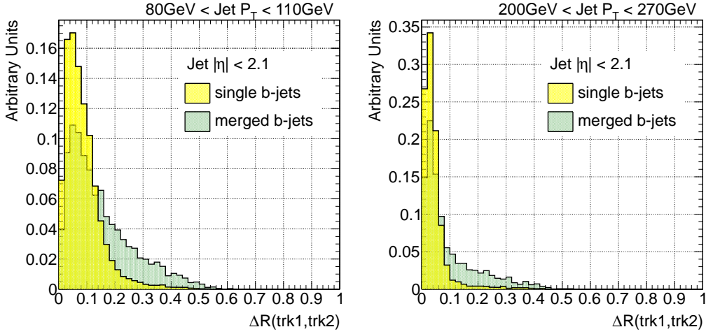
Figure 5.10: Distribution of \Delta R between leading tracks for single and merged b -jets from 80 GeV to 110 GeV (left) and 200 GeV to 270 GeV (right).
