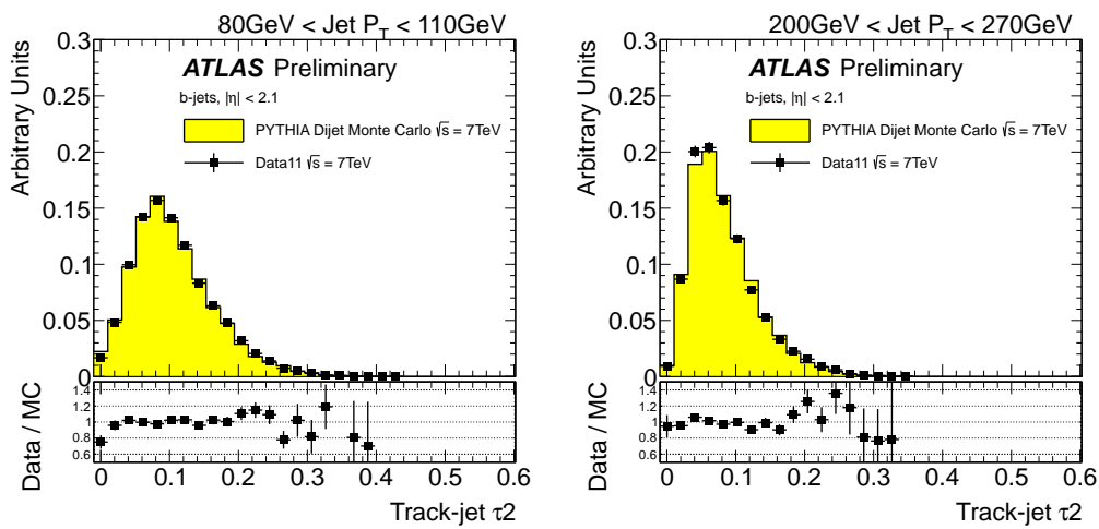
Figure 5.23: Distribution of \tau_2 in two different jet p_T bins, for experimental data collected by ATLAS during 2011 (solid black points), and simulated data (filled histograms). The ratio data over simulation is shown at the bottom of each plot.
