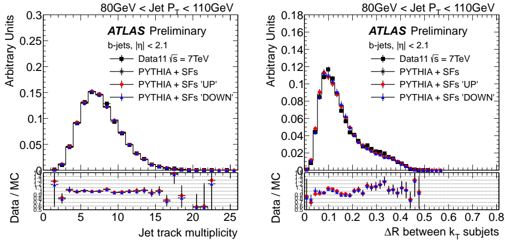
Figure 6.7: The effect of a variation in the b -tagging Scale Factors on the tracking variables distributions. Scale Factors were varied up (down) by 1-sigma to evaluate the systematic uncertainty from this source. The ratio data over MC is shown for MC PYTHIA with SFs varied up (circles) and down (triangles).
