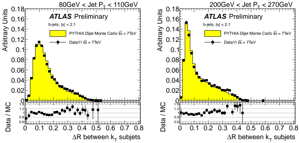
Figure 5.21: Distribution of the \Delta R between the axes of the two k_t subjects in the jet in 2 different jet p_T bins, for experimental data collected by ATLAS during 2011 (solid black points), and simulated data (filled histograms). The ratio data over simulation is shown at the bottom of each plot.
