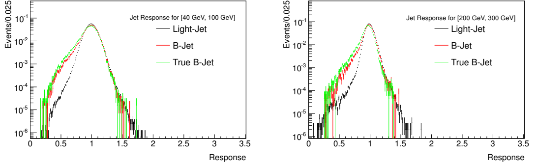
Figure 8.2 The response function for b -tagged jets (red), true b -jets (green) and untagged jets (black), as calculated using MC samples in the truth p_T ranges [40, 100] GeV (left) and [200, 300] GeV (right).
