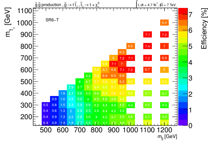
Figure 9.16 The signal efficiency for gluino mediated stop pair production in the (m_{\tilde{g}}, m_{\tilde{t}_1}) plane for the pMSSM gluino-stop model, for the signal region SR6-T.
