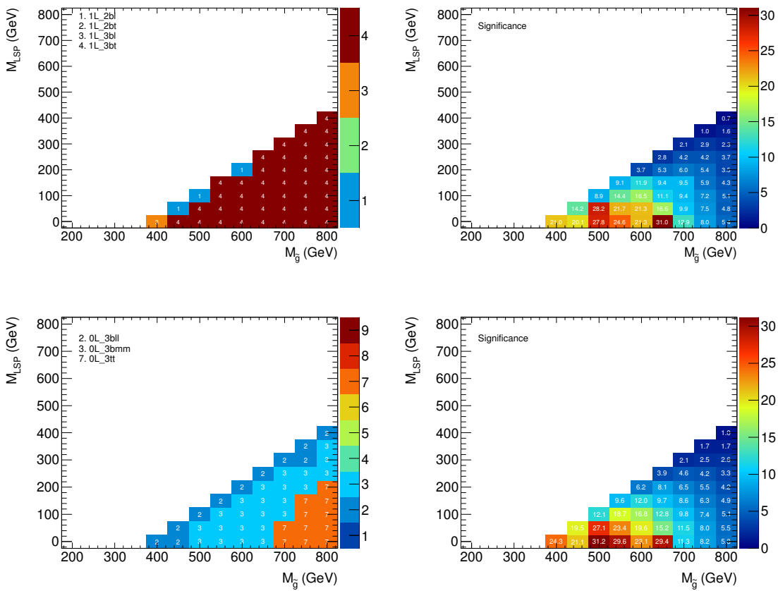
Figure 7.9 Top left: best selection cuts using the 1-lepton selection. The 3 b -tag analysis is found to be the best strategy for more than 95% of the mass plane for the Gtt topology. Top right: the significance for the best set of cuts at a given point for the 1-lepton. Bottom left: best selection cuts using the 0-lepton selection. Bottom right: 0-lepton significance after requiring a higher total jet multiplicity in combination with looser b -tagging operating points, and enhanced m_{\text{eff}} and E_T^{\text{miss}} cuts, while keeping the SM prediction yield around \mathcal{O}(10) events. The resulting 0-lepton selections are found to be competitive with the 1-lepton selection sensitivity.
