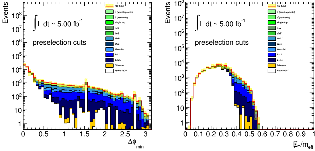
Figure 7.4 Distribution of \Delta\phi_{min} (left) and E_T^{miss}/m_{eff} (right), after requiring the event to have the leading jet with p_T > 130 GeV, E_T^{miss} > 130 GeV and at least three jets with p_T > 30 GeV, in the zero-lepton selection.
