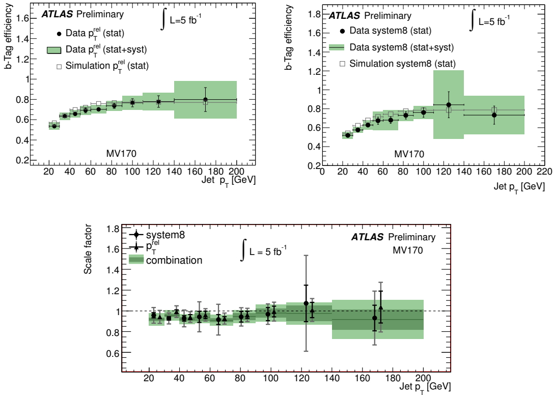
Figure 5.6 Top: The b -tag efficiency in data and simulation for the MV1 tagging algorithm at \text{OP} = 70\% efficiency as a function of the jet p_T , obtained with the p_T^{\text{rel}} (left) and the System8 (right) methods. Bottom: The data-to-simulation scale factor for the MV1 tagging algorithm at \text{OP} = 70\% efficiency as a function of the jet p_T , obtained from the p_T^{\text{rel}} and System8 results. The dark green band represents the statistical uncertainty of the combined scale factor while the light green band shows the total uncertainty. The data points showing the p_T^{\text{rel}} and System8 measurements have been separated a little along the x -axis to make the plot more readable.
