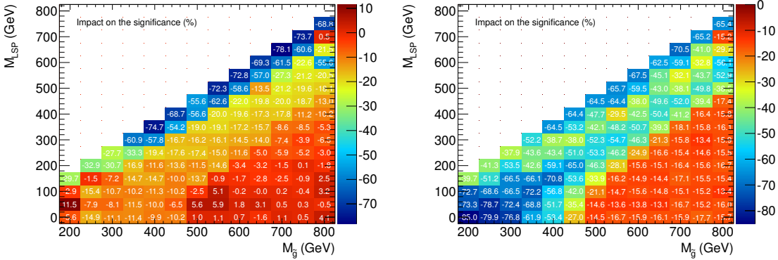
Figure 7.7 Impact on the significance after removing the E_T^{\text{miss}}/m_{\text{eff}} cut (left) and the \Delta\phi_{\text{min}} > 0.4 cut (right) for Gbb topologies. For the regions where the 3 b -jet analysis performs the best (95% of the mass plane, see Figure 7.6), the degradation in sensitivity is found to be from 10 % to 50 % depending on the mass-splitting and topology. Similar performance has been observed for Gtb and Gtt topologies.
