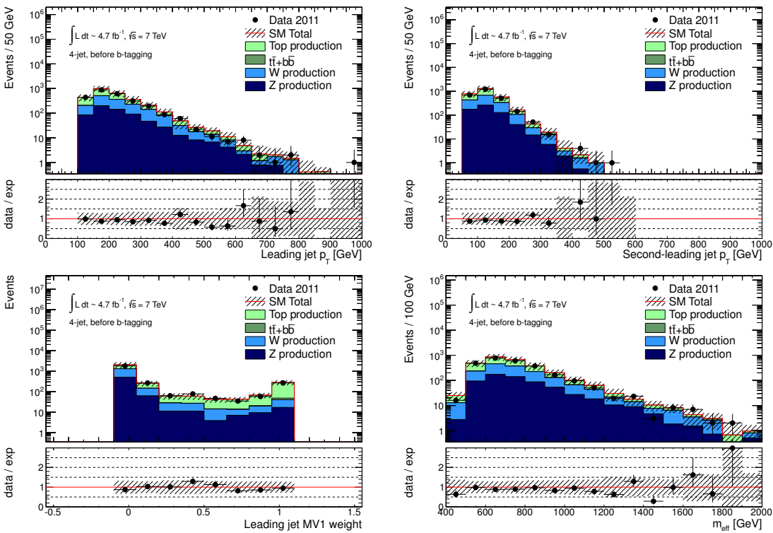
Figure 8.6 From top to bottom, left to right: the distributions of the leading jet p_T , the second leading jet p_T , the leading jet MV1 b -tagger weight and m_{\text{eff}} after applying the cuts #1 – 13 (for the 4-jet selection and E_T^{\text{miss}} > 160 GeV) as introduced in Table 7.11 (i.e., before the b -tagging requirement).
