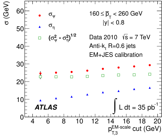
Figure 6.7 Standard deviations \sigma_\psi^{\text{calo}} , \sigma_\eta^{\text{calo}} and [(\sigma_\psi^2 - \sigma_\eta^2)^{\text{calo}}]^{1/2} as a function of the upper p_{T,3}^{\text{EM-scale}} cut, for R = 0.6 anti- k_t jets with \bar{p}_T = 160 - 260 GeV. The increase of the soft radiation contribution to \sigma_\psi^{\text{calo}} and \sigma_\eta^{\text{calo}} cancels in the squared difference, and within statistical uncertainties it remains constant up to p_{T,3}^{\text{EM-scale}} \simeq 20 GeV.
