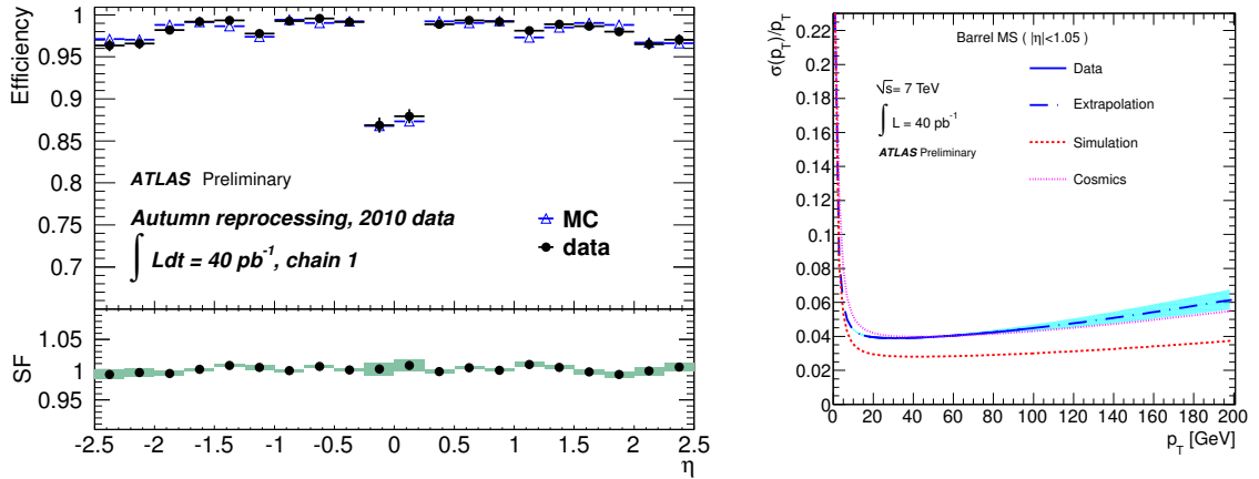
Figure 5.2 Left: Efficiencies for CB plus ST muons, obtained from data (dots) and Monte Carlo simulation (open triangles) as function of muon \eta and integrated over a p_T range of 20 GeV - 100 GeV, using STACO-family algorithms. The scale factor correction and its corresponding uncertainty are shown in the lower part of the figure. Right: Muon momentum resolution curve in collision data and simulation as a function of the muon p_T , for the pseudo-rapidity region |\eta| < 1.05 . The solid blue line shows determinations based on data and is continued as dashed line for the extrapolation to p_T ranges not accessible due to statistics. The shaded band represents the sum in quadrature of the statistical and systematic uncertainties. The curve obtained from cosmic ray data is overlaid for comparison.
