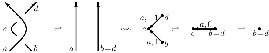
FIGURE 6. Second Reidemeister move \leftrightarrow R2+R0
