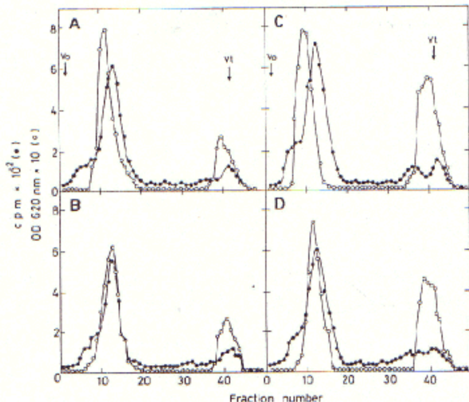
Fig. 1 Bio-Gel P4 chromatography of \beta(1-2) glucans accumulated in vivo by R. fredii strains. A) o, R. fredii USDA191 cellular glucans accumulated in vivo ; ●, glucans formed in vitro . B) o, R. fredii USDA191 cellular glucans accumulated in vivo after alkaline treatment (0.5 N NaOH, 80 min., 100°C); ●, glucans formed in vitro . C) o, R. fredii USDA257 cellular glucans accumulated in vivo ; ●, glucans formed in vitro . D) o, R. fredii USDA257 cellular glucans accumulated in vivo after alkaline treatment (0.5 N NaOH, 80 min., 100°C); ●, glucans formed in vitro . Carbohydrate assays and counting of radioactivity were carried out as described in Materials and Methods. Bio-Gel P4 columns (78 x 1.8 cm) were eluted with 0.1 M pyridine-acetate buffer (pH 5.5). Fractions of 1.5 ml were collected. Vo is the void vol.; Vt is the total vol.
