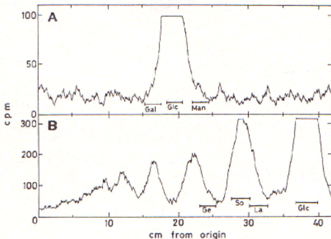
Fig. 4 Characterization of cyclic \beta (1-2) glucan formed in vitro . In vitro synthesis of cyclic \beta (1-2) glucan was carried out with inner membranes of R. fredii USDA257 as described in Materials and Methods. Glucan was purified by Bio-Gel P4 chromatography and subjected to total or partial acid hydrolysis as described in Materials and Methods. A) Descending paper chromatography of total acid hydrolysis products. The chromatogram was developed with solvent A. B) Descending paper chromatography of partial acid hydrolysis products. Chromatograms were developed with solvent B. Standards: Gal: galactose; Glc: glucose; Man: mannose; Ge: gentiobiose; So: sophorose; La: laminaribiose
