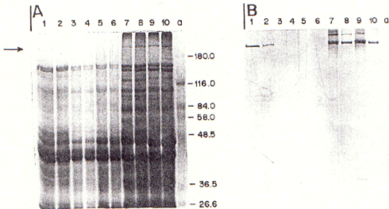
Fig. 3. Polyacrylamide gel electrophoresis of inner membranes of R. fredii strains. Inner membranes were incubated with UDP- ^{14}\text{C} -glucose at 12°C. Reactions were stopped by addition of 10% TCA, and precipitates were subjected to sodium dodecyl sulfate-polyacrylamide gel electrophoresis and fluorography as indicated in Materials and Methods. Proteins were stained with Coomassie blue (A), and radioactivity was detected by fluorography (B). For a chase experiment (even-numbered lanes), 2 mM non-radioactive UDP-glucose was added after a 10 min. incubation, and the reaction was stopped after 10 min. Lanes 1 and 2: Strain HH303; lanes 3 and 4: Strain ndvB Rf19; lanes 5 and 6: strain N101; lanes 7 and 8: strain USDA191; lanes 9 and 10 strain USDA257. a: molecular weight standards. Numbers on the left indicate molecular masses of standards (in kDa). The arrow indicates the migration position of the A. tumefaciens 235 kDa intermediate protein.
