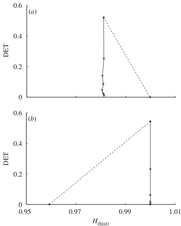
Figure 4. DET as a function of H^{(\text{hist})} , as evaluated in De Micco et al. (2008), for both randomization procedures applied to: (a) LOG; (b) TWB. Squares and dashed lines, discretization; circles and solid lines, skipping.
