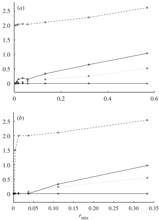
Figure 2. Recurrence plots quantifiers as functions of r_{\text{mix}} : (a) LOG; (b) TWB. Squares, RR; circles, L; up triangles, DET; right triangles, ENTR.
